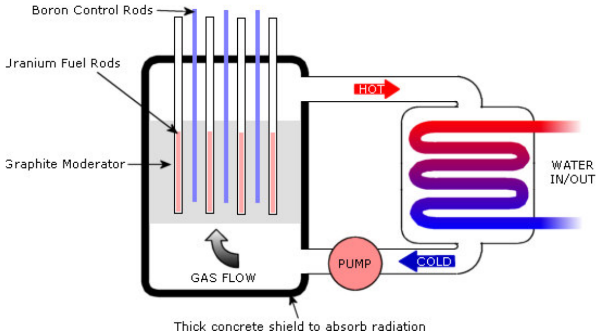
Gareth Jones 2003 – How a Nuclear Powerstation works
